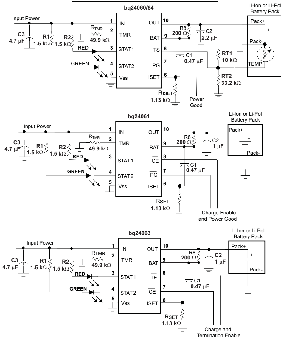
Figure 16. Application Circuits
